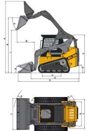
Vertical lift path
