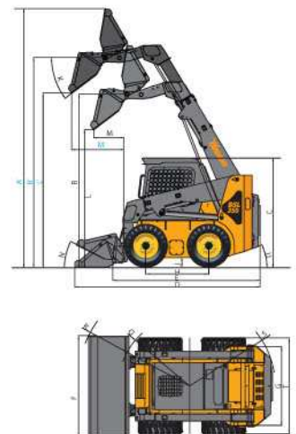
Radial lift path(EX)
